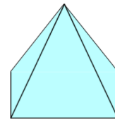
Square-based pyramid
